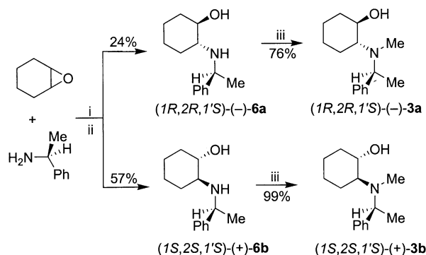
Scheme 3. Reagents and conditions: i. LiClO 4 /MeCN, reflux, 18 h; ii. separation of diastereomers by column chromatography; iii. HCO 2 H/HCHO, reflux, 4 h.
