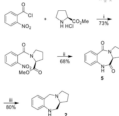
Scheme 2. Reagents and conditions: i. Et 3 N/CH 2 Cl 2 , 0 °C; ii. Fe/AcOH, 110 °C; iii. LiAlH 4 /THF, −10 °C→reflux temp., N 2 .
