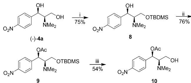
Scheme 5. Reagents and conditions: i. t BuMe 2 SiCl, Et 3 N, DMAP/CH 2 Cl 2 , 25 °C, 18 h; ii. AcCl, Et 3 N, DMAP/CH 2 Cl 2 , 0–25 °C, 5 h; iii. n Bu 4 NF/THF, 25 °C, 40 min.
