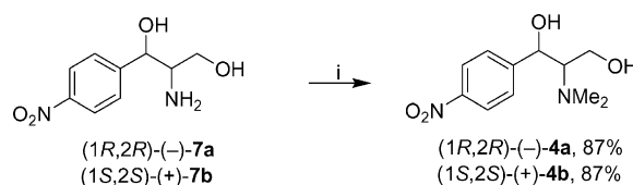
Scheme 4. Reagents and conditions: HCO 2 H/HCHO, reflux, 4 h.
