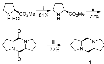
Scheme 1. Reagents and conditions: i. 50% K 2 CO 3 , 0 °C; ii. 105 °C; iii. LiAlH 4 /THF, room temp.→reflux temp., N 2 .
