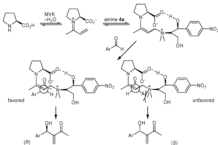
Figure 1. Transition state for the (–)- 4a /L-proline-catalyzed MBH reaction between aromatic aldehyde and MVK.
